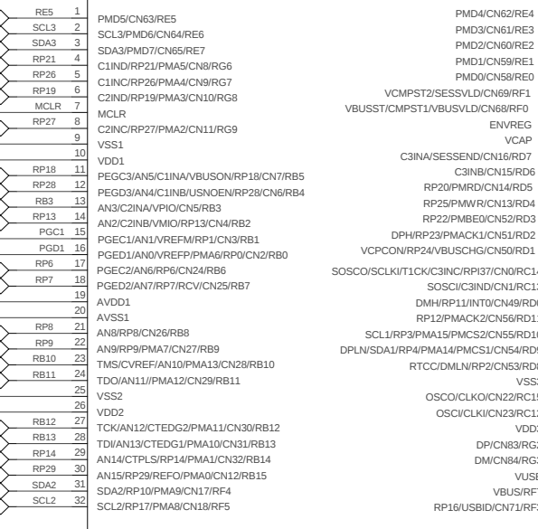
PIC24FJ256GB206_TQFP64
