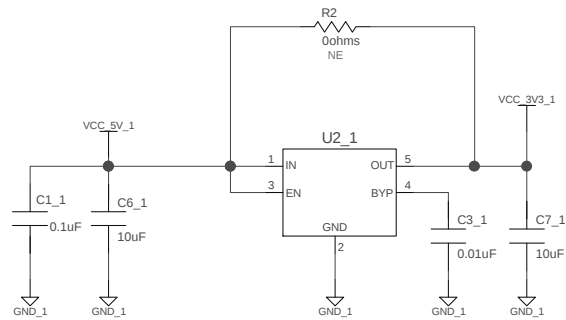
SPX3819M5-L-3-3 MIC5504-3.3YM5-TR
