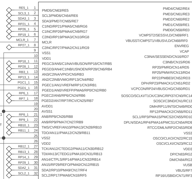
PIC24FJ256GB206_TQFP64
